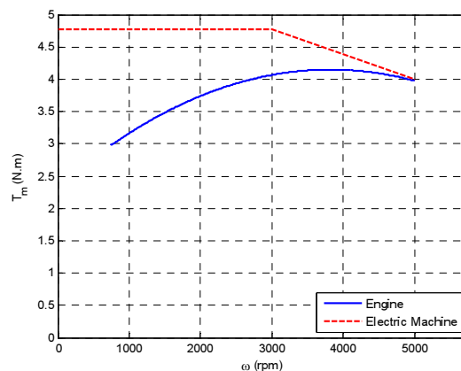
Fig. 7. Comparison of torque speed characteristics of scaled engine and the selected motor.
