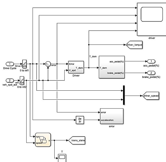
Figure 7: Driver block structure.
