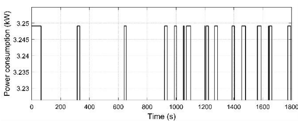
Figure 4: Power consumption of the compressor
