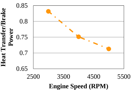
Figure 9: Experimental Heat Transfer to Brake Power Ratio
