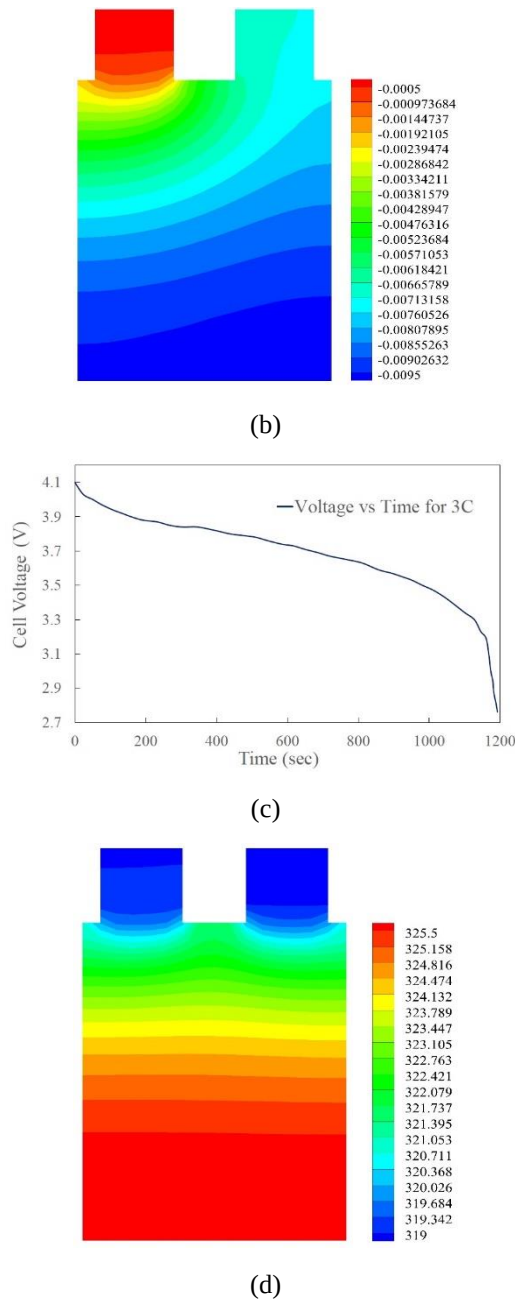
Figure 5: Contour plot of phase potential for (a) positive electrode, (b) negative electrode, (c) cell voltage variation and (d) maximum cell temperature for 3C rate of discharging.
