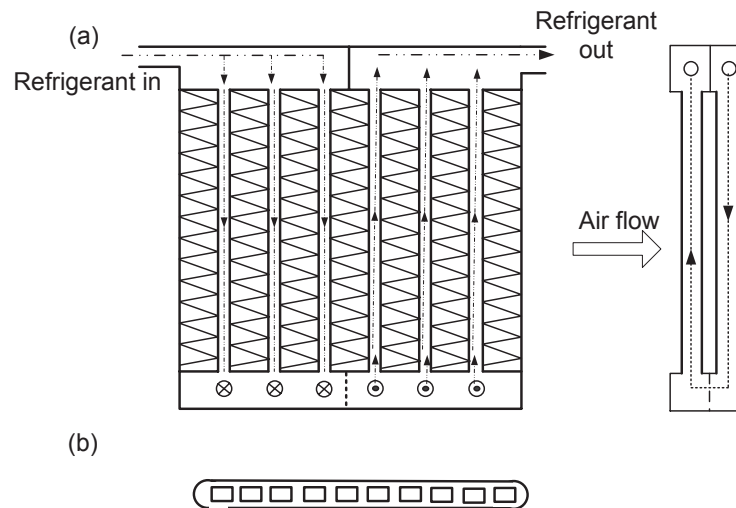
Fig. 2. The schematic view of a parallel flow evaporator. (a) Front view of parallel flow evaporator. (b) mini-channel cross sections
